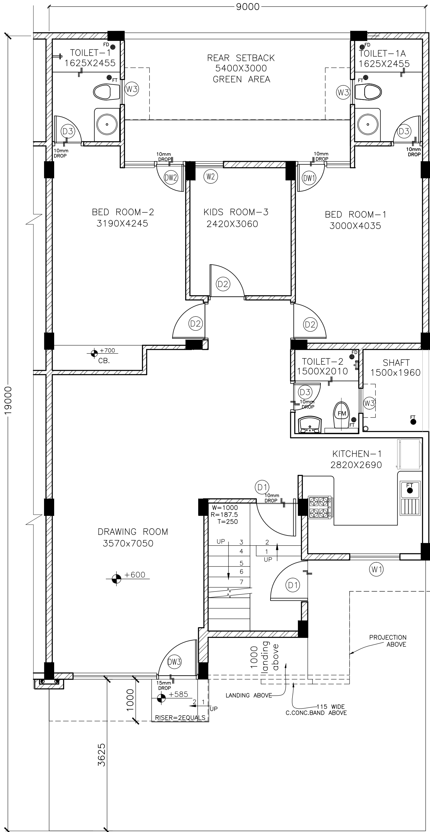
171 SQM_ WF _(SITE PLAN)
