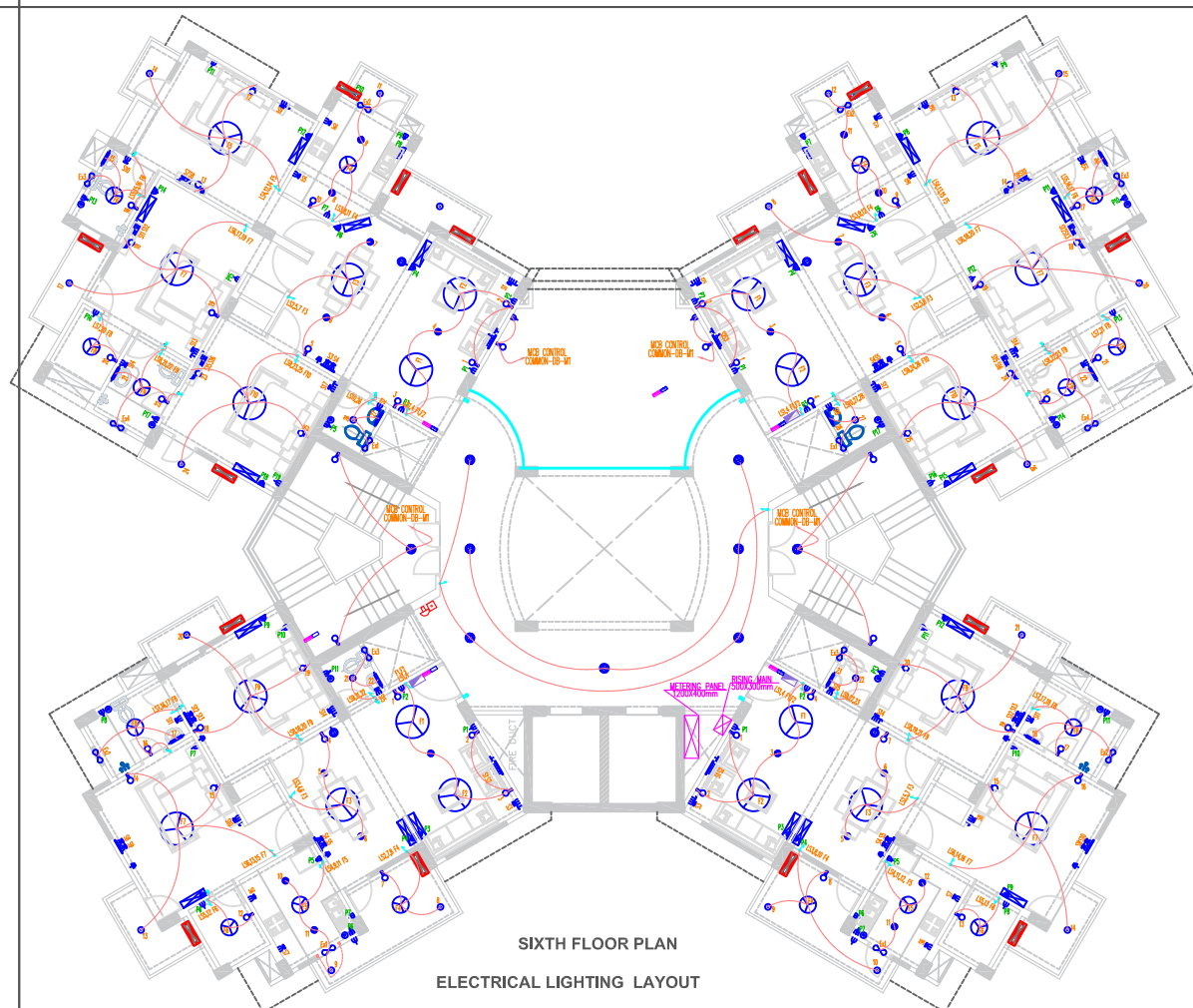
SIXTH FLOOR PLAN ELECTRICAL LIGHTING & CONDUITING LAYOUT
