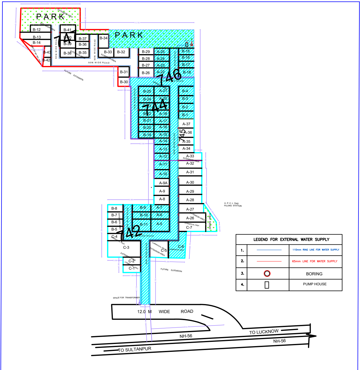
WATER SUPPLY PLAN
