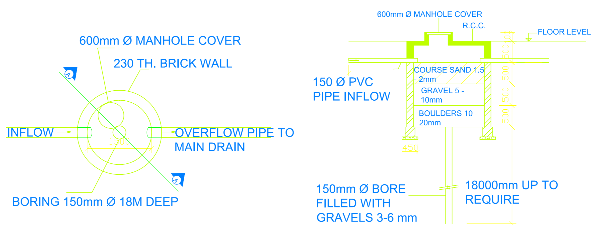
RAIN WATER HARVESTING DETAIL
