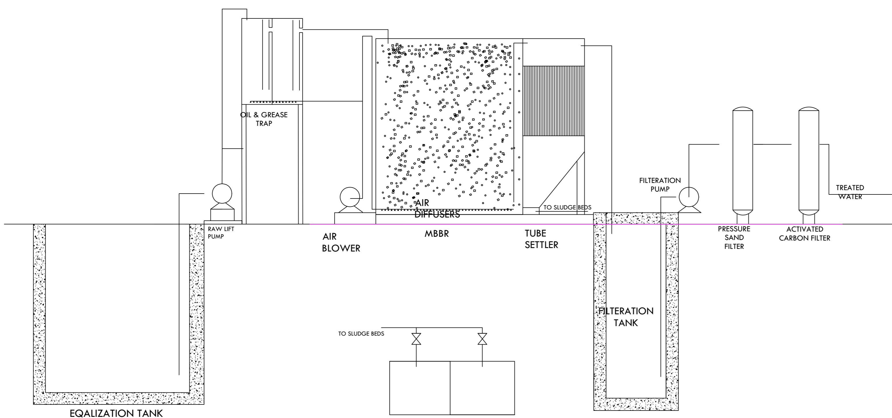
SERVICES PLAN - STP
