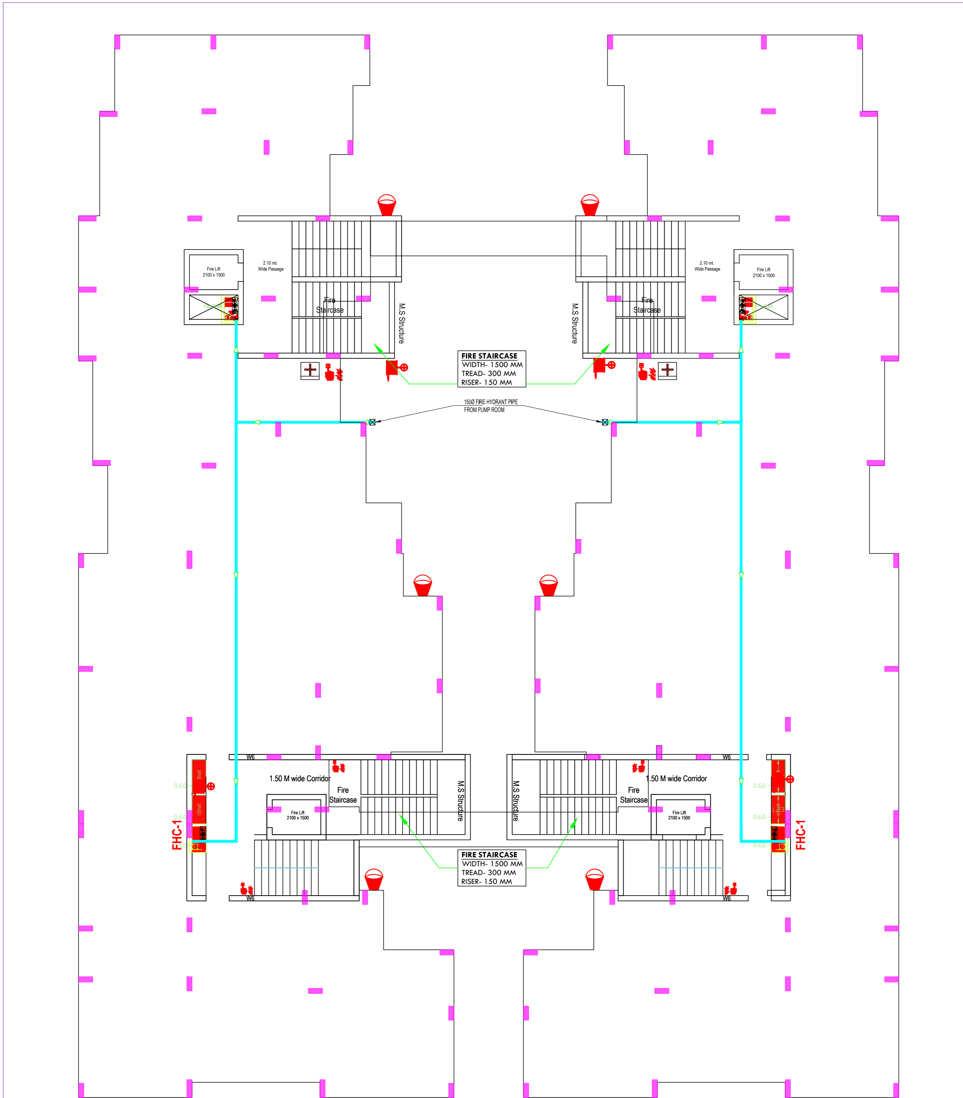
FIRE FIGHTING PLAN
