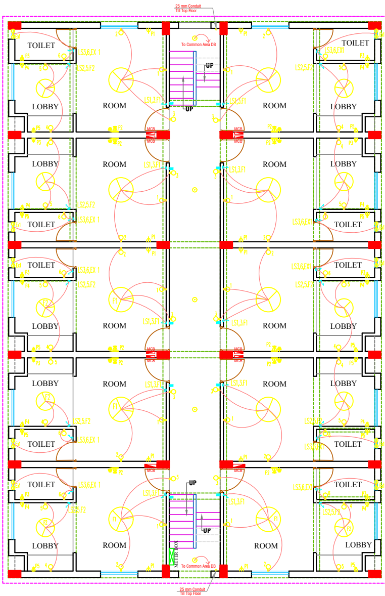
GROUND FLOOR PLAN ELECTRICAL LIGHTING CIRCUIT
