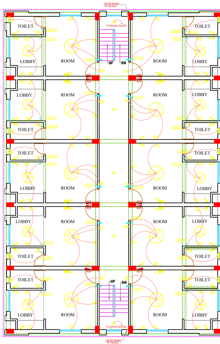
TYPICAL FLOOR PLAN ELECTRICAL LIGHTING CIRCUIT
