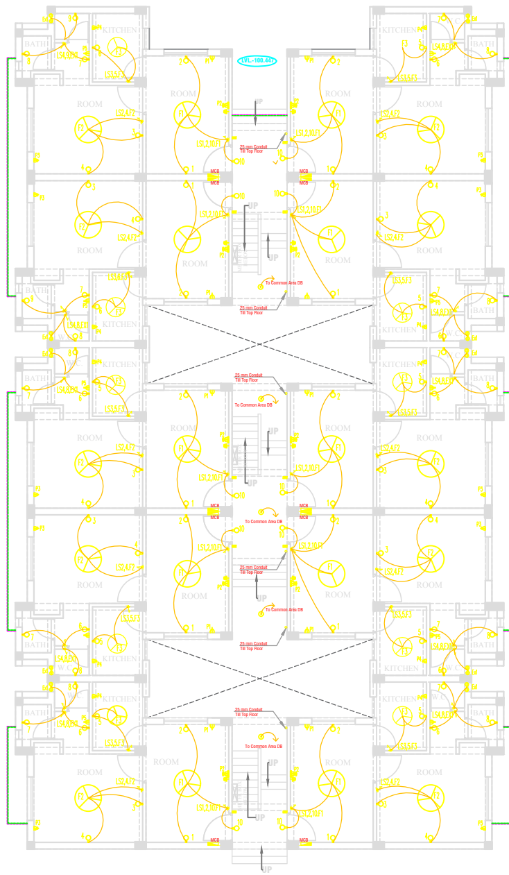
GROUND FLOOR PLAN ELECTRICAL LIGHTING CIRCUIT LAYOUT
