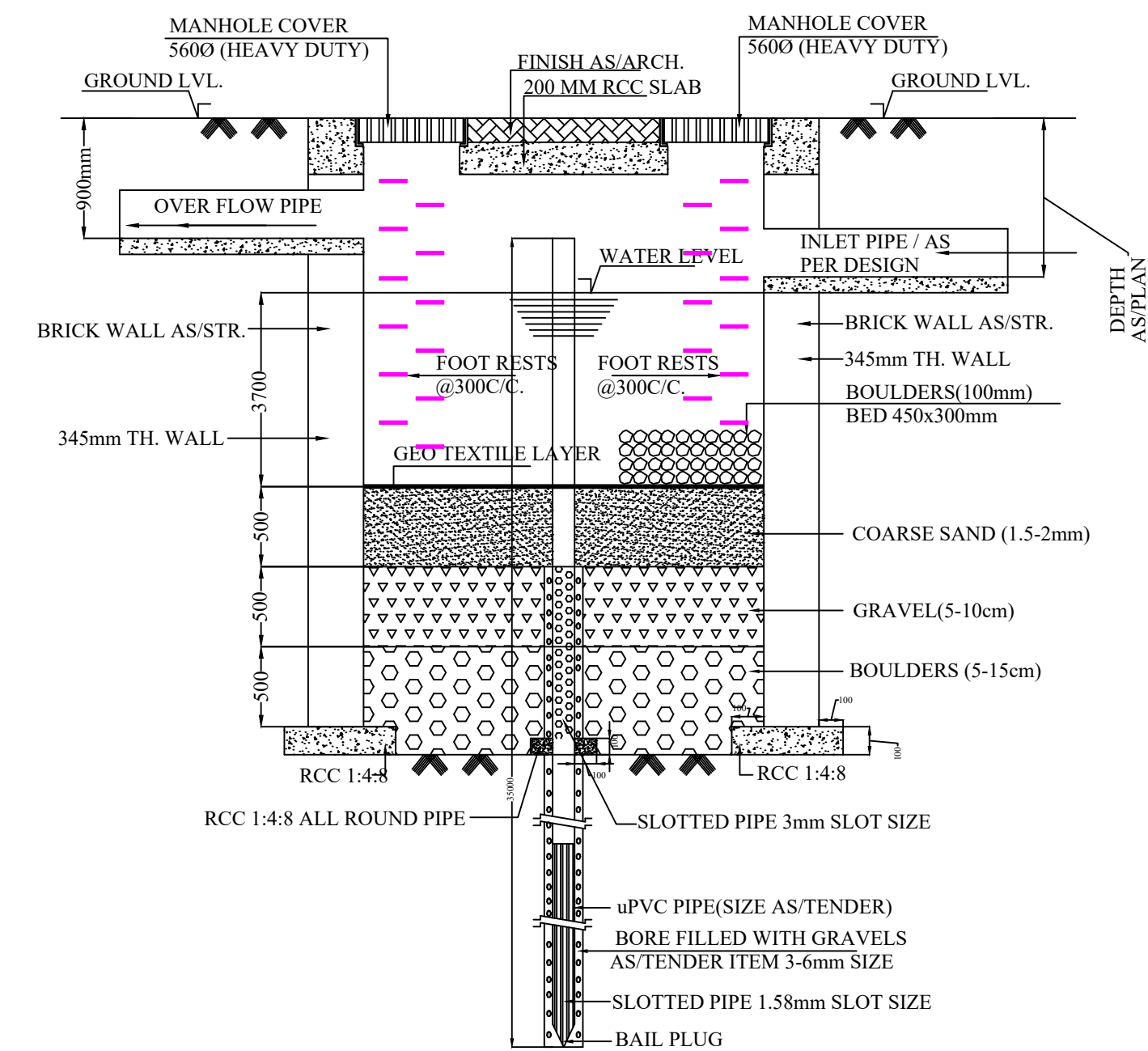
SECTION TYPICAL DETAIL 3.000M DIA HARVESTING DETAILS
