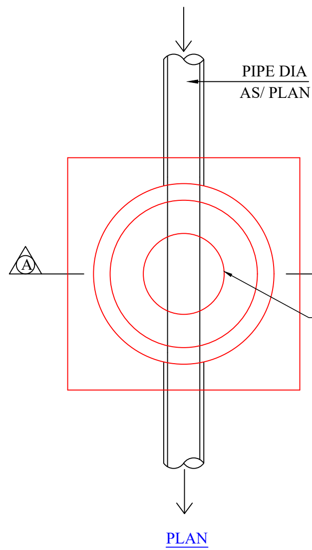
PLAN CIRCULAR MANHOLE 900 DIA (CPWD SPECIFICATIONS-1977 CLAUSE - 20.4 FIG.107)
