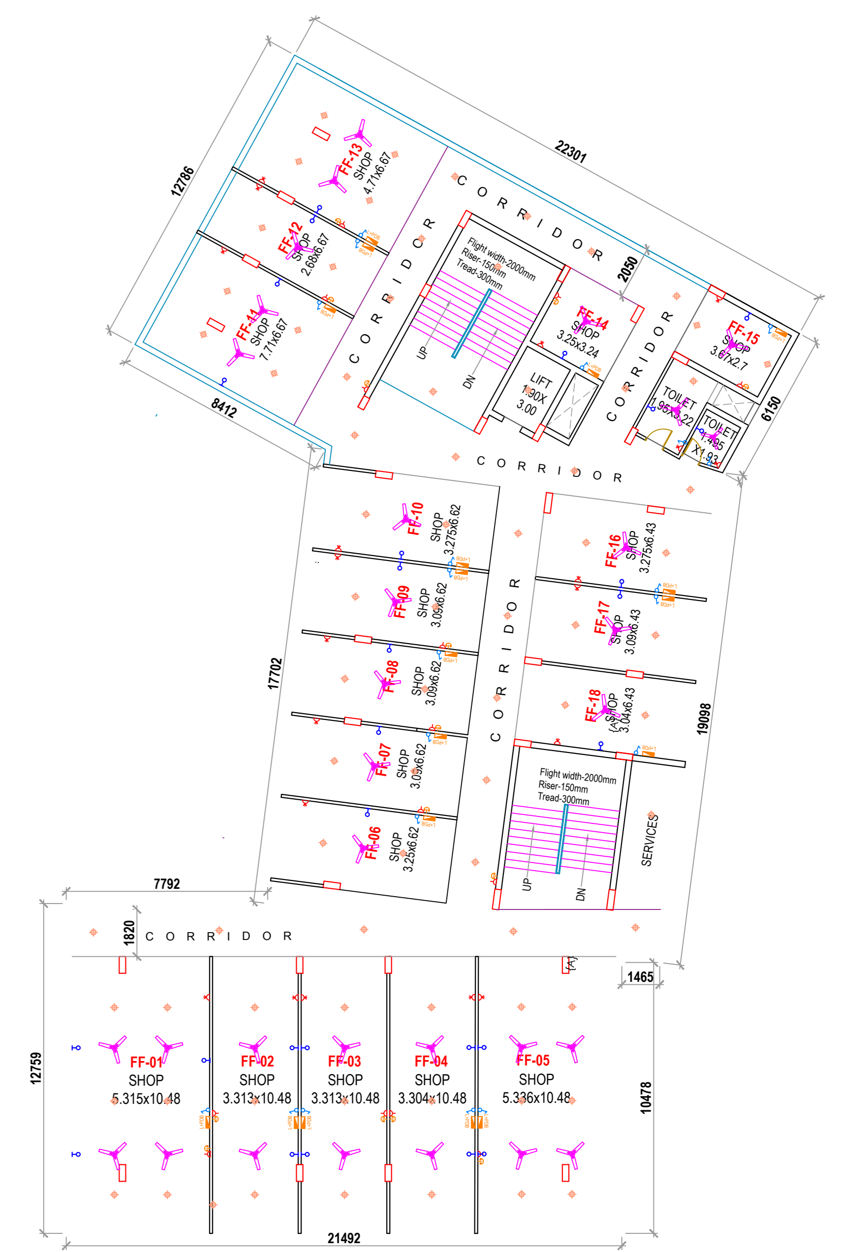
FIRST FLOOR PLAN (SCALE 1:200)
