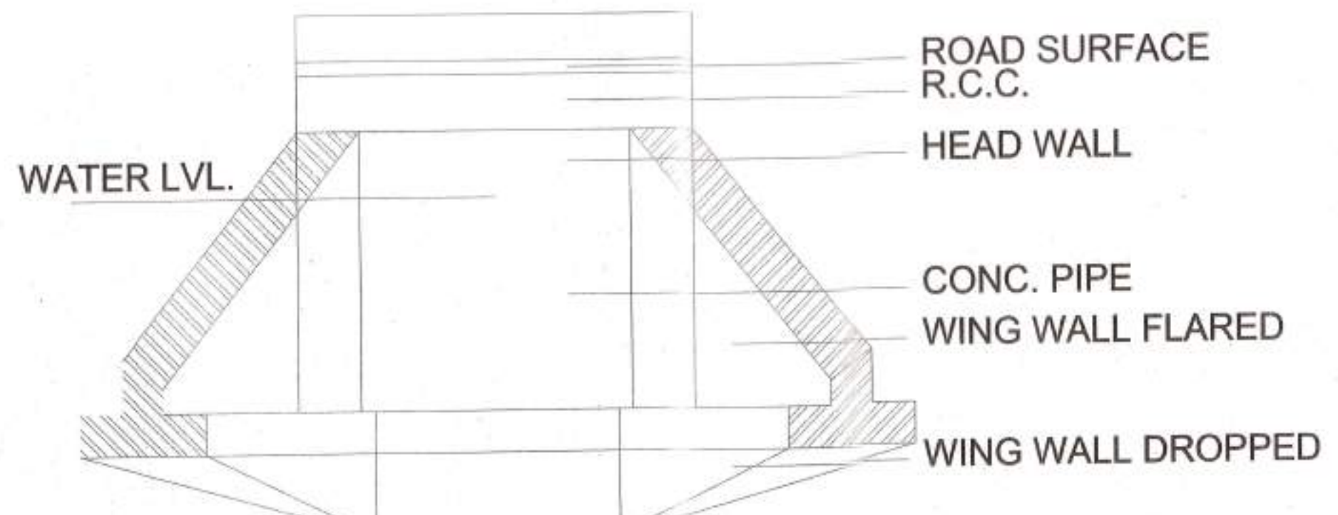
TYPICAL CULVERT DETAIL
