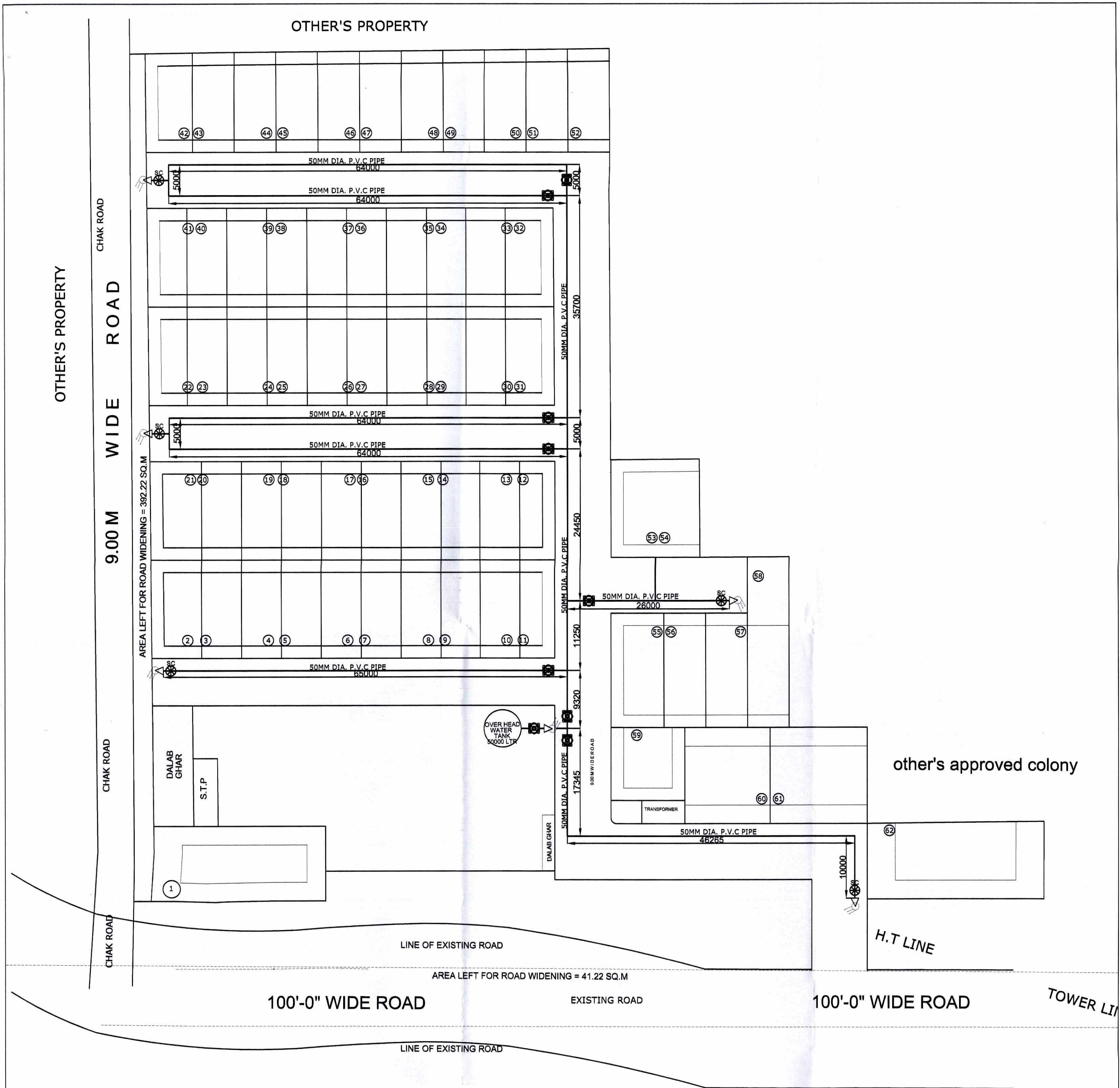
WATER SUPPLY LAYOUT PLAN
