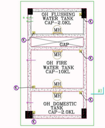
TYPICAL PLANS & DETAILS OF OVERHEAD TANKS
