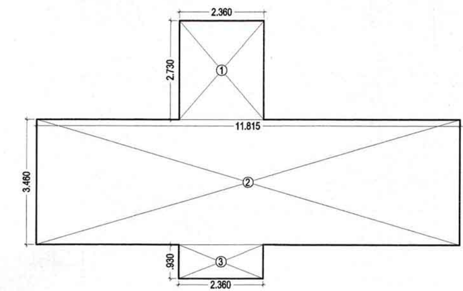
MACHINE ROOM & O.H.T. AREA CALCULATION
