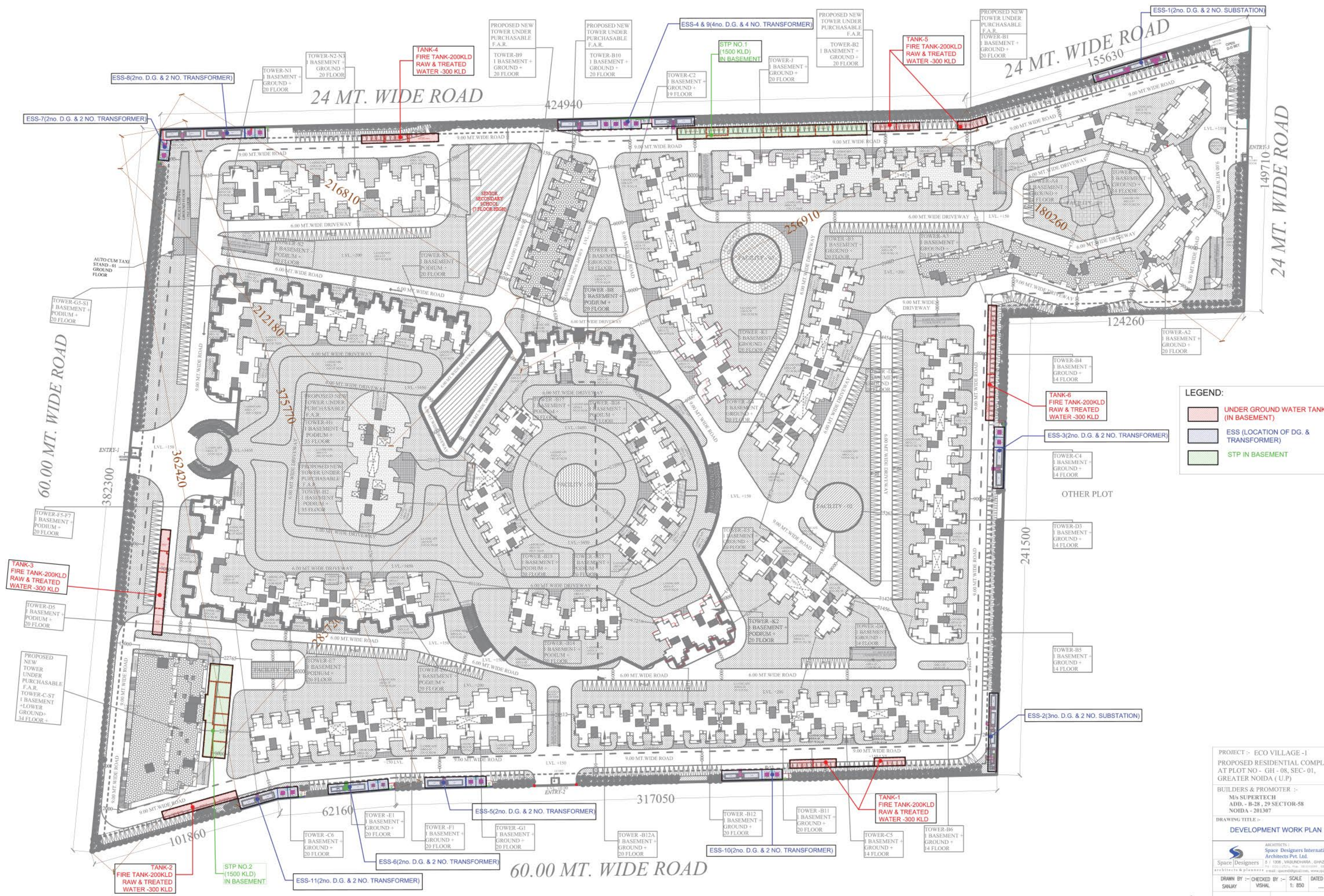
SITE PLAN
