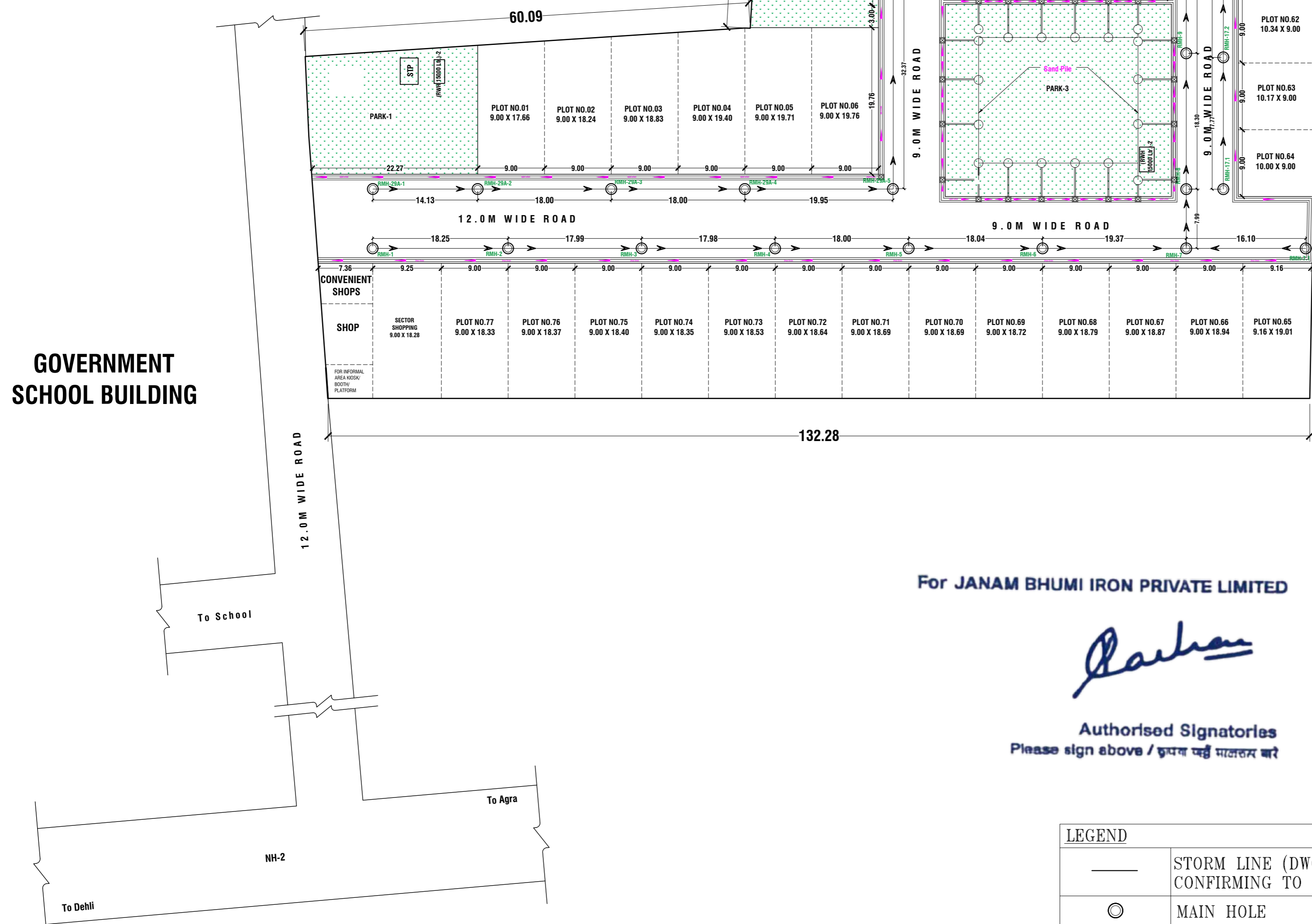
Storm Water Layout Plan
