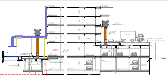
TYPICAL SITE SECTION BUILDING HEIGHT IS BASEMENT + PODIUM + 24 FLOORS
