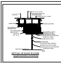
DETAIL OF RAIN WATER HARVESTING SYSTEM
