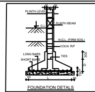
FOUNDATION DETAILS
