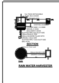
DETAIL OF RAIN WATER HARVESTING SYSTEM
