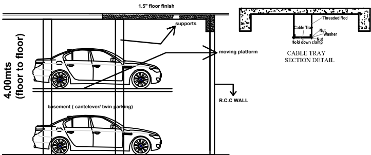
MECHANIZED PARKING SECTION DETAIL
