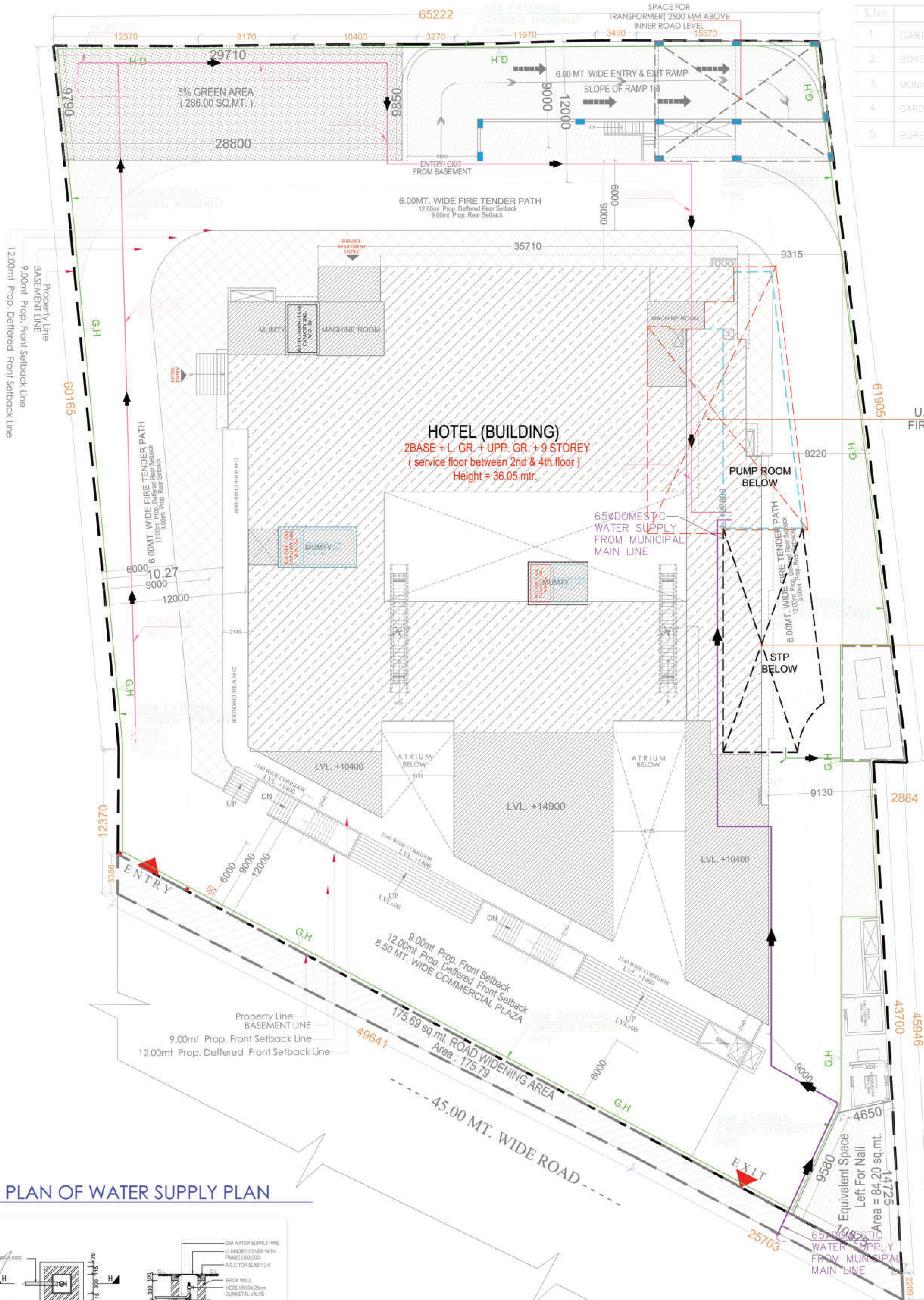
PLAN OF WATER SUPPLY PLAN
