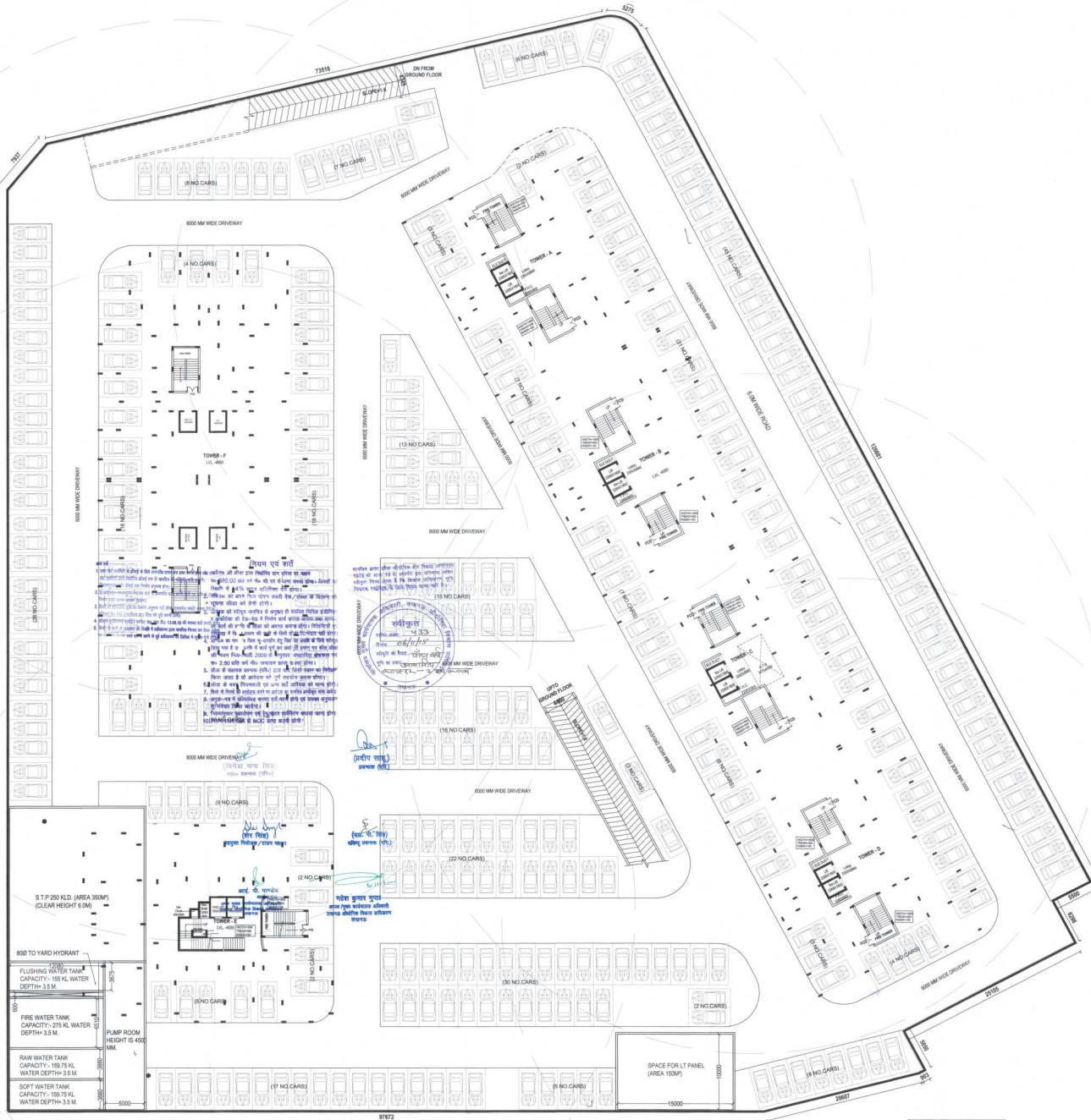
BASEMENT PLAN (NO. OF CARS-356NOS) (AREA-15667.06 SQ.MT.)
