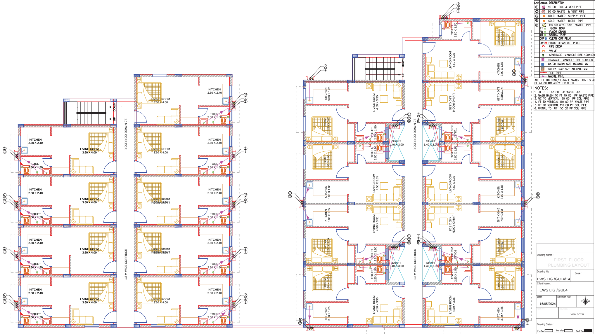
FIRST FLOOR PLUMBING LAYOUT
