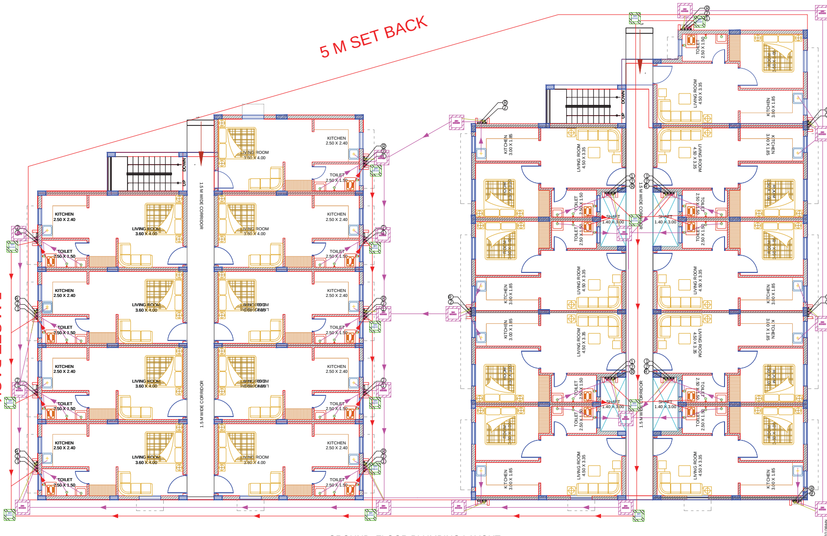
GROUND FLOOR PLUMBING LAYOUT
