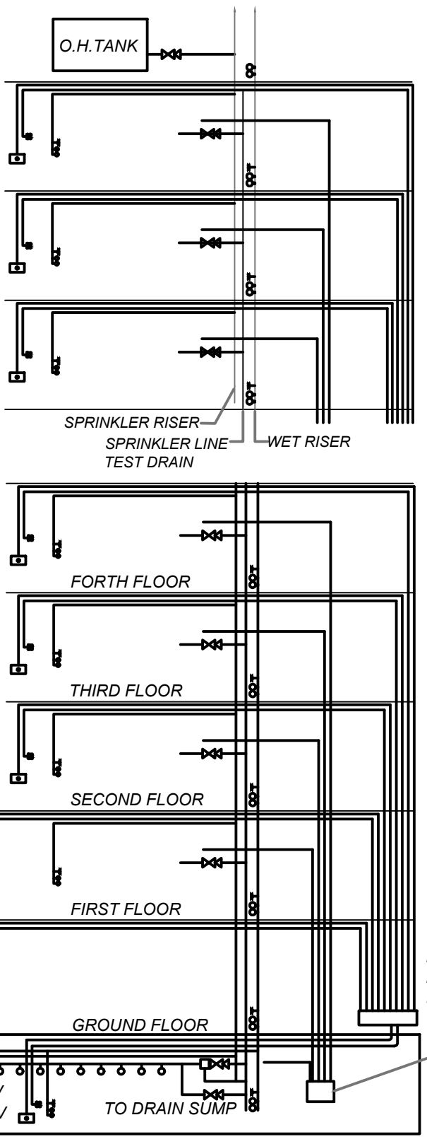
TYPICAL ARRANGEMENT OF WET RISER AND TOTAL SPRINKLER SYSTEM OF BUILDING OTHER THAN APARTMENT EXCEEDING 30.0 M IN HEIGHT
