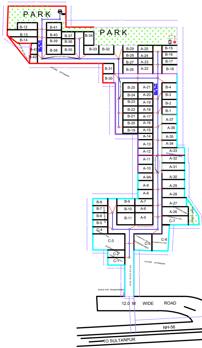
SEWER PLAN FOR VIDHI ESTATE EXTENSION
