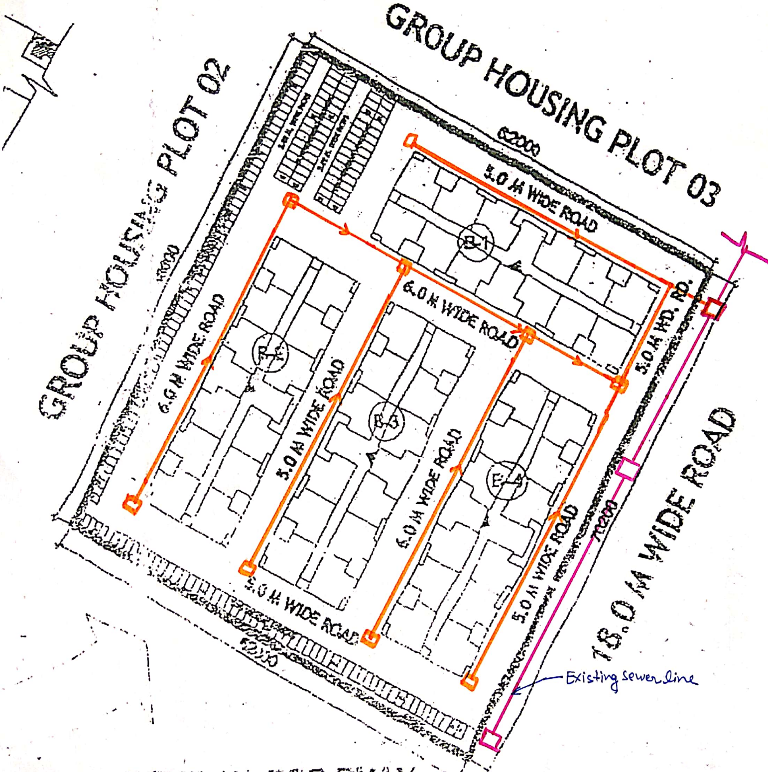
LAYOUT PLAN FOR DRAINAGE DETAIL - A
