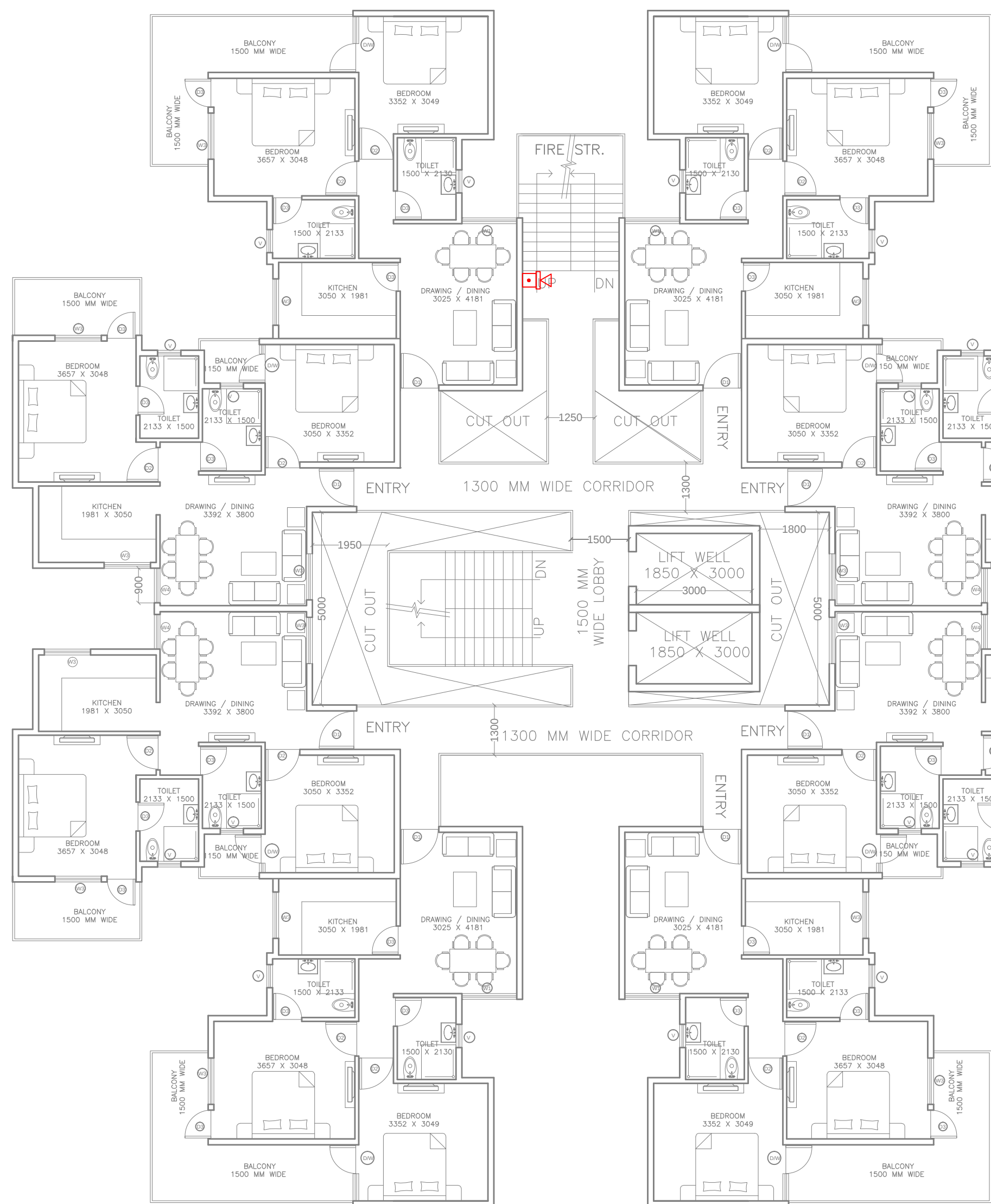
TYPICAL PLAN
