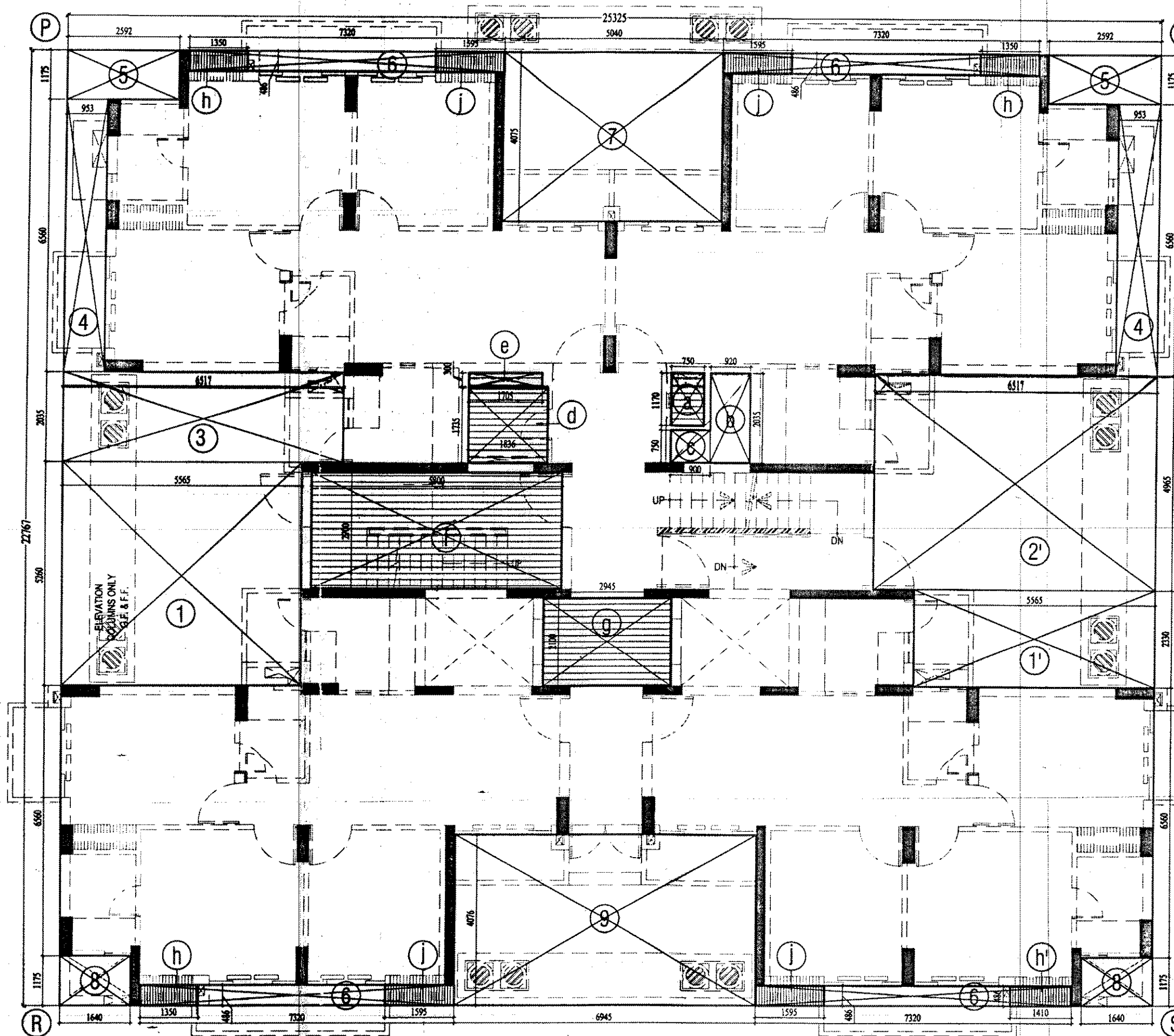
AREA ENVELOPE PLAN AT GROUND FLOOR
