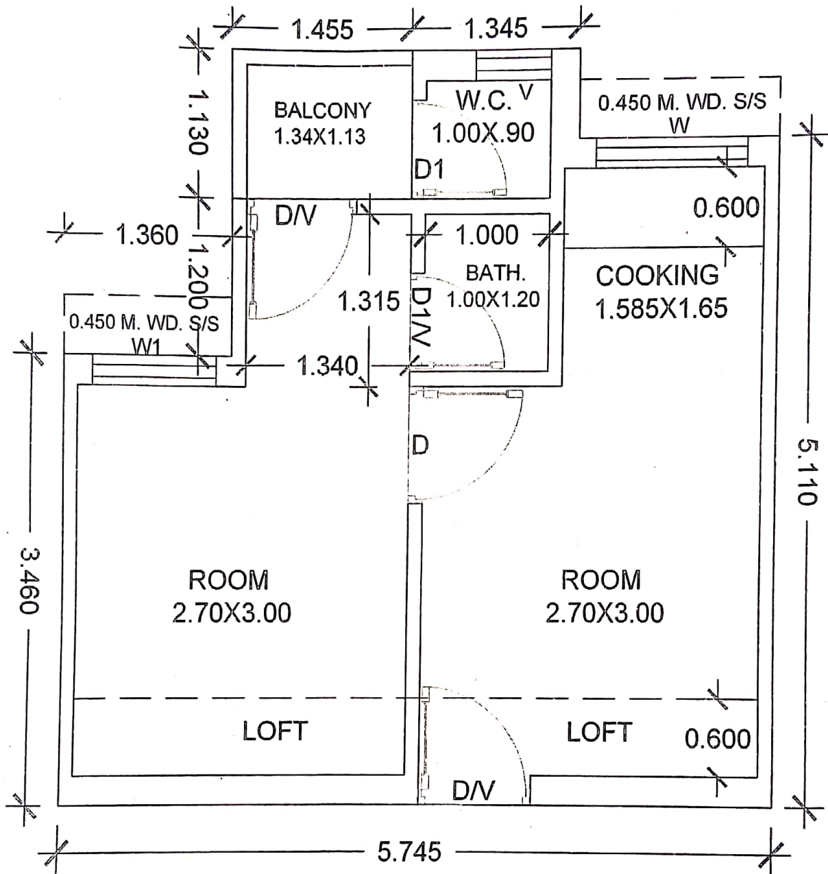
UNIT PLAN
