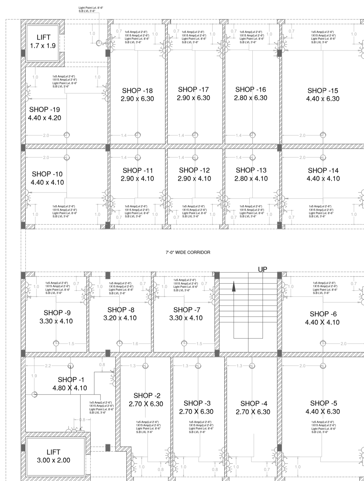
GROUND FLOOR PLAN ELECTRICAL PLAN
