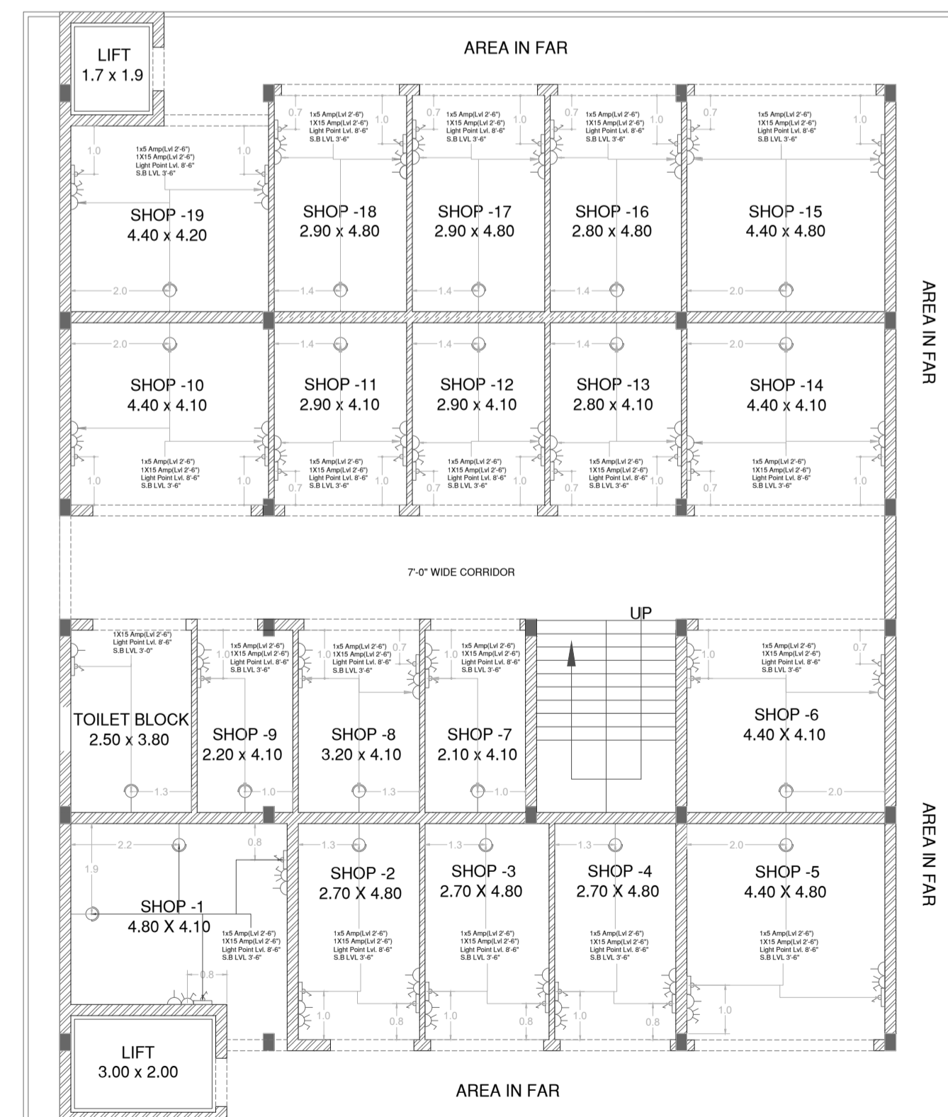
FIRST FLOOR PLAN ELECTRICAL PLAN
