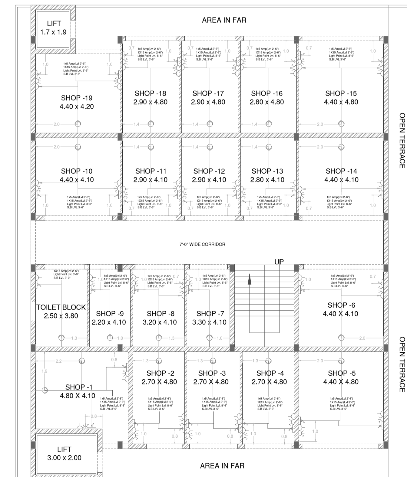
SECOND FLOOR PLAN ELECTRICAL PLAN
