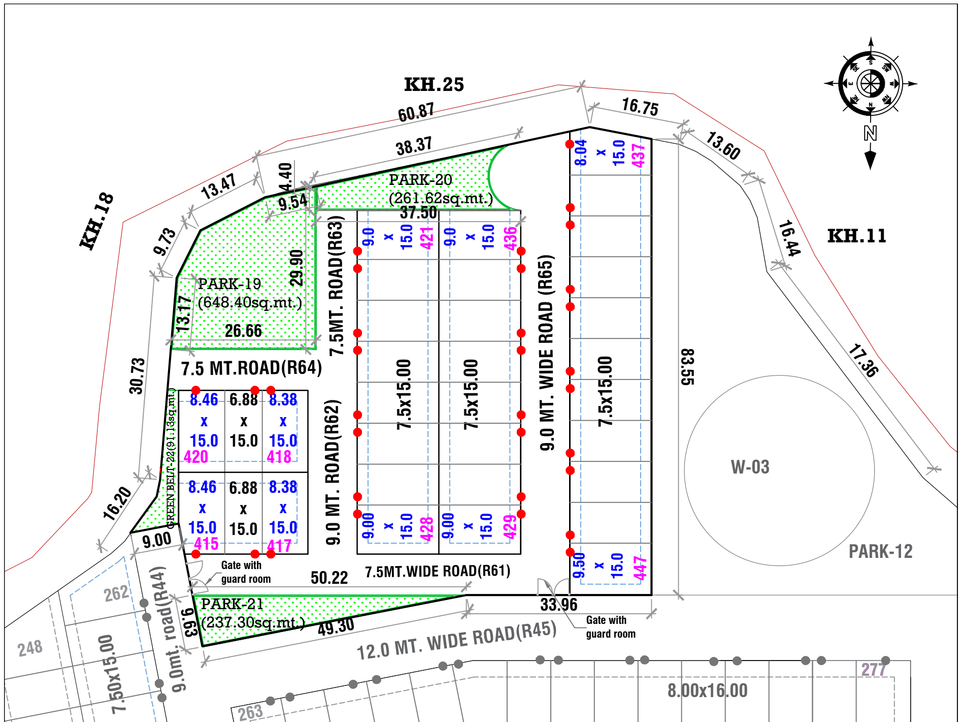
DEVELOPMENT LAYOUT-ELDECO INNER CIRCLE
