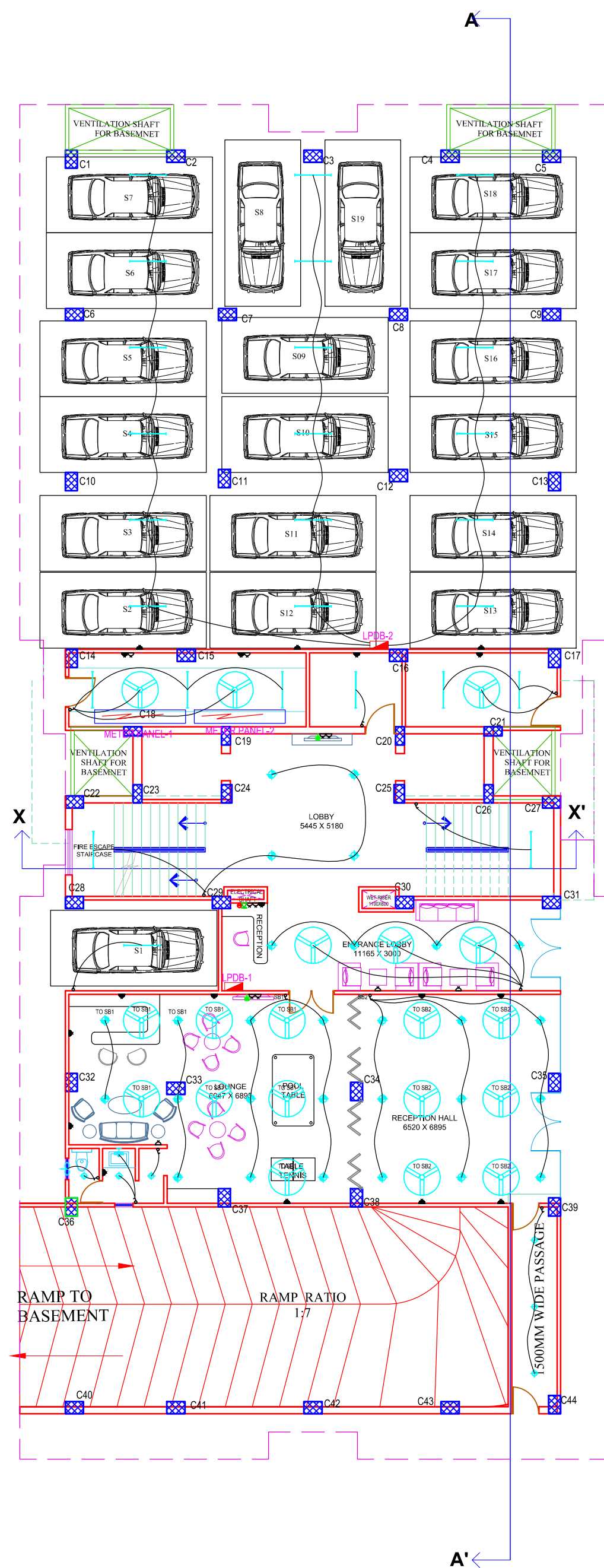
STILT PLAN
