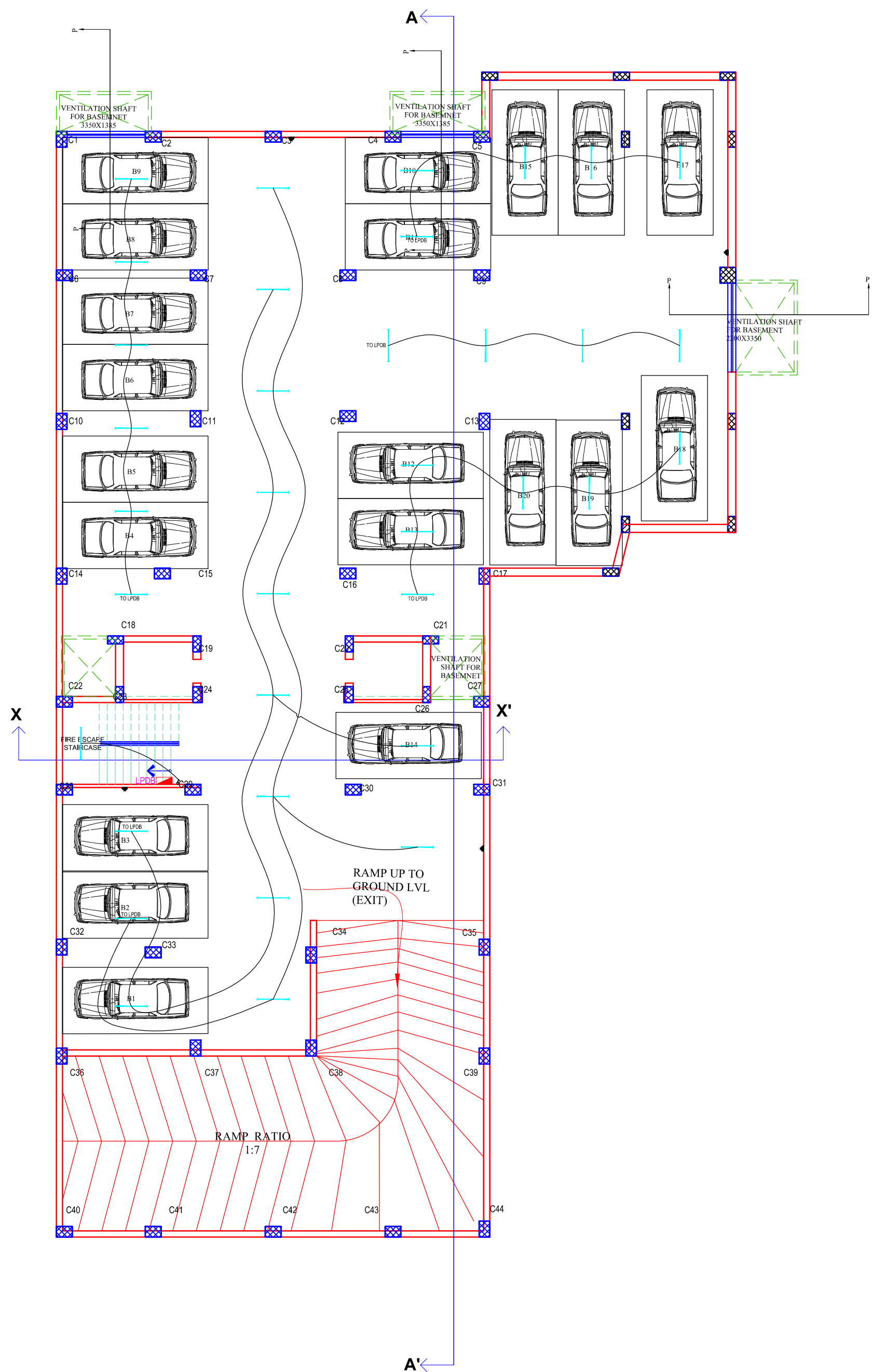
BASEMENT PLAN
