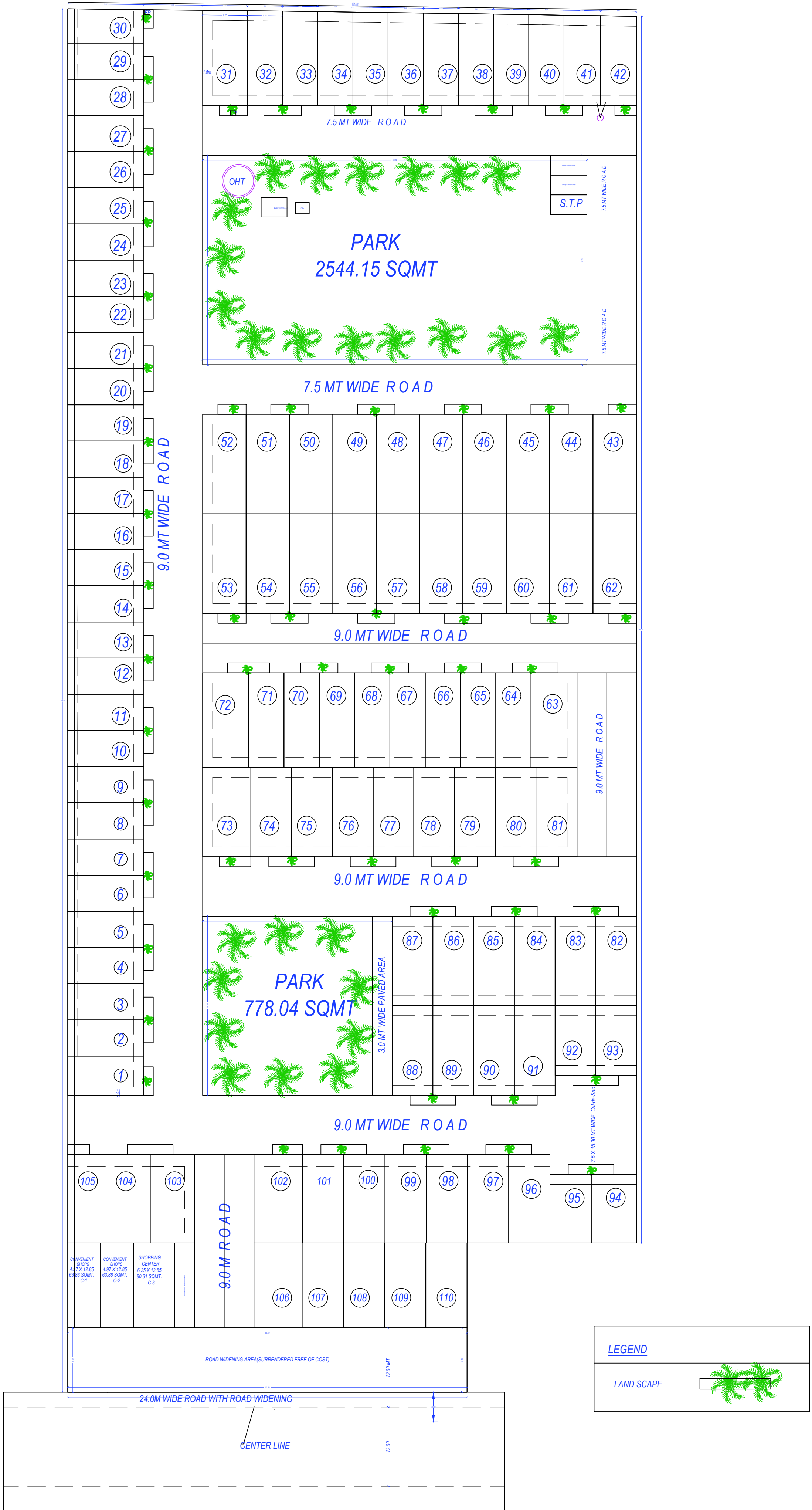
LANDSCAPE PLAN
