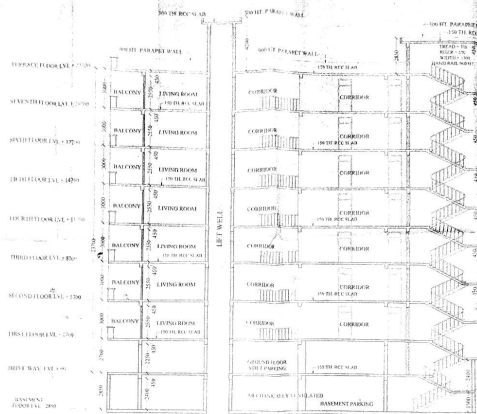
SECTION AT X-X
