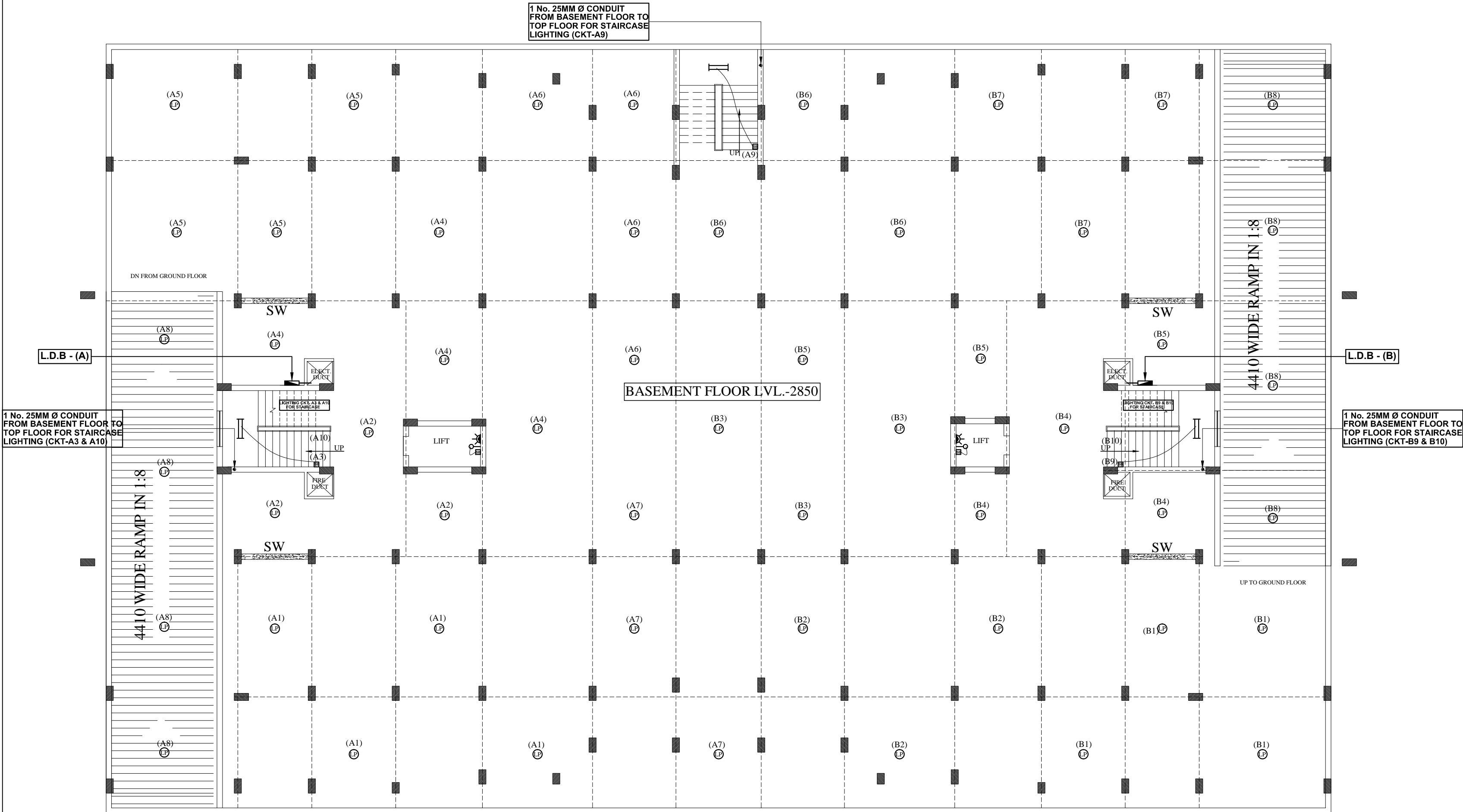
BLOCK-A BASEMENT FLOOR PLAN
