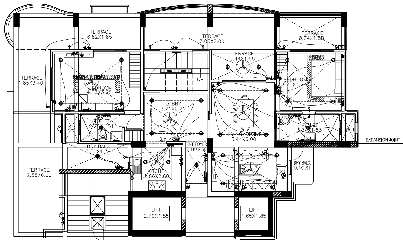
TENTH FLOOR PLAN (ELECTRICAL LAYOUT)
