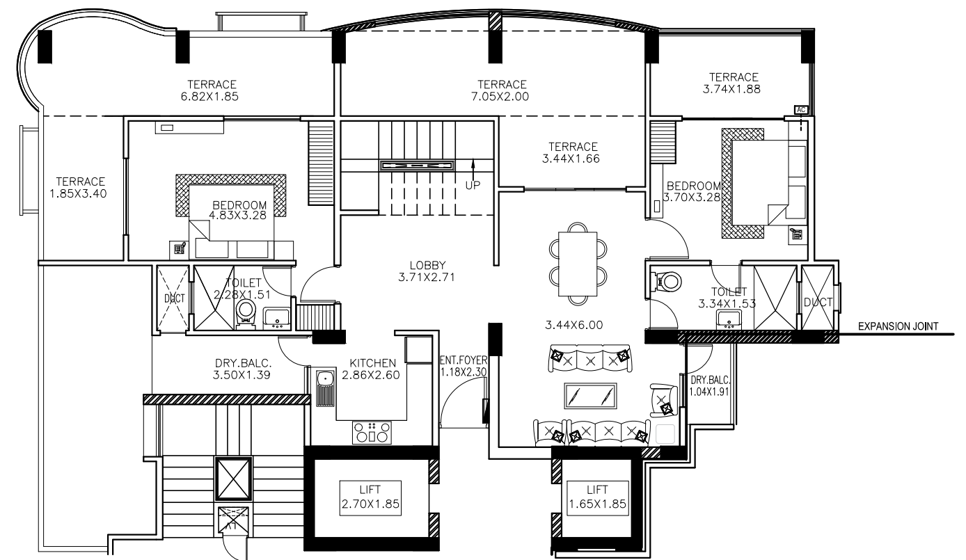
TENTH FLOOR PLAN (FURNITURE LAYOUT)
