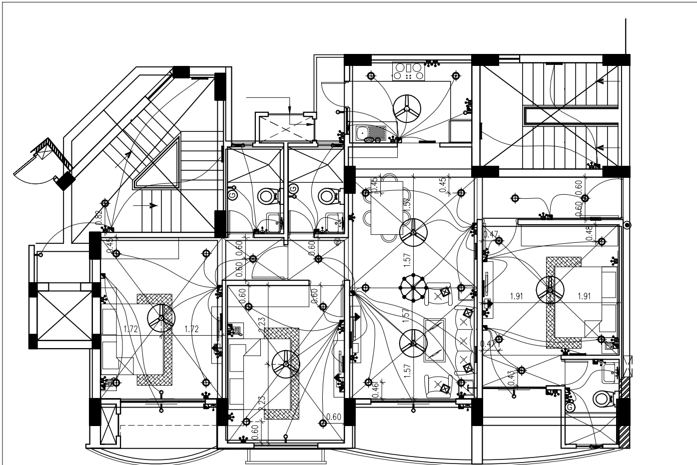
ELECTRICAL LAYOUT
