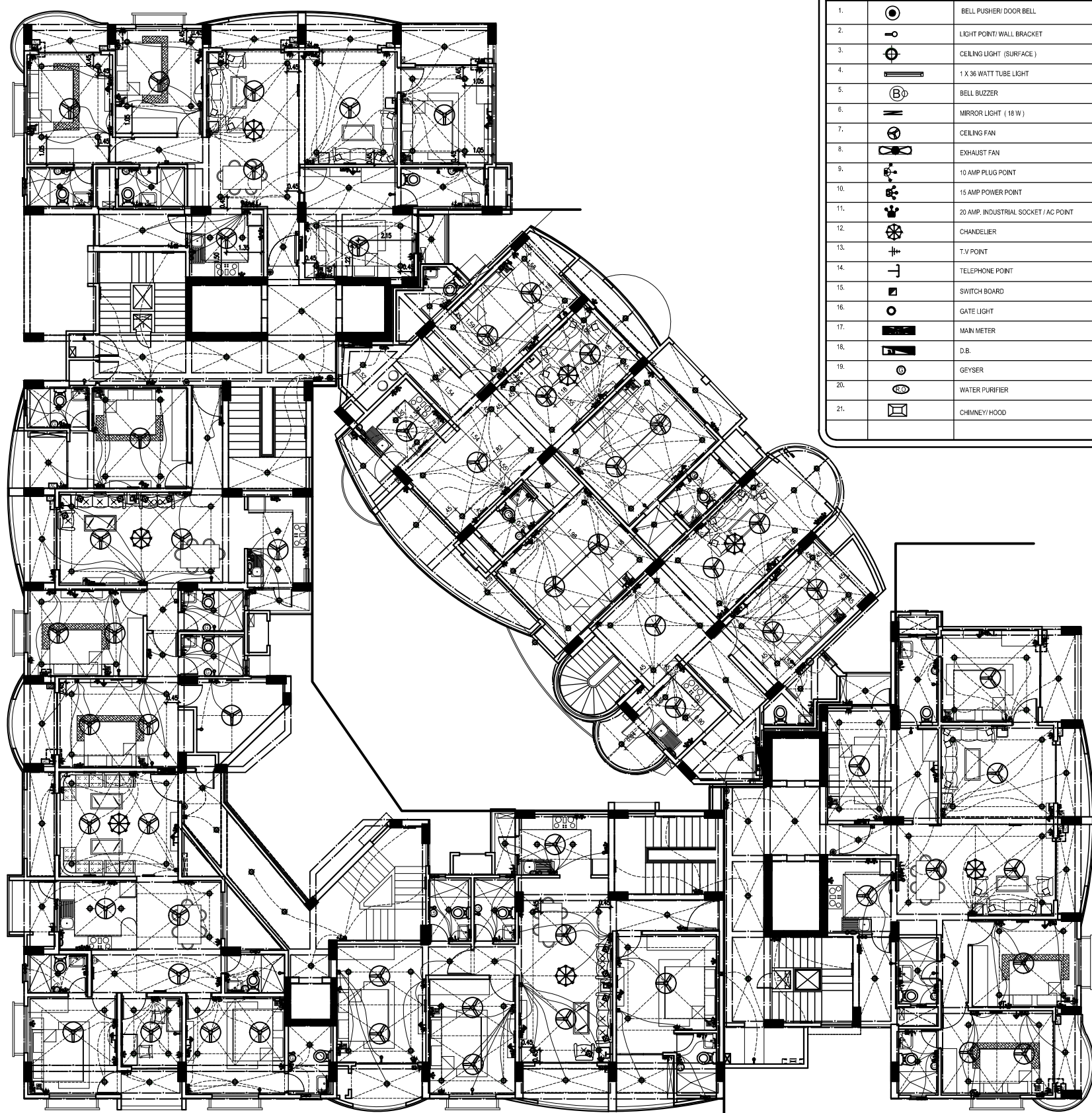
NINE FLOOR PLAN
