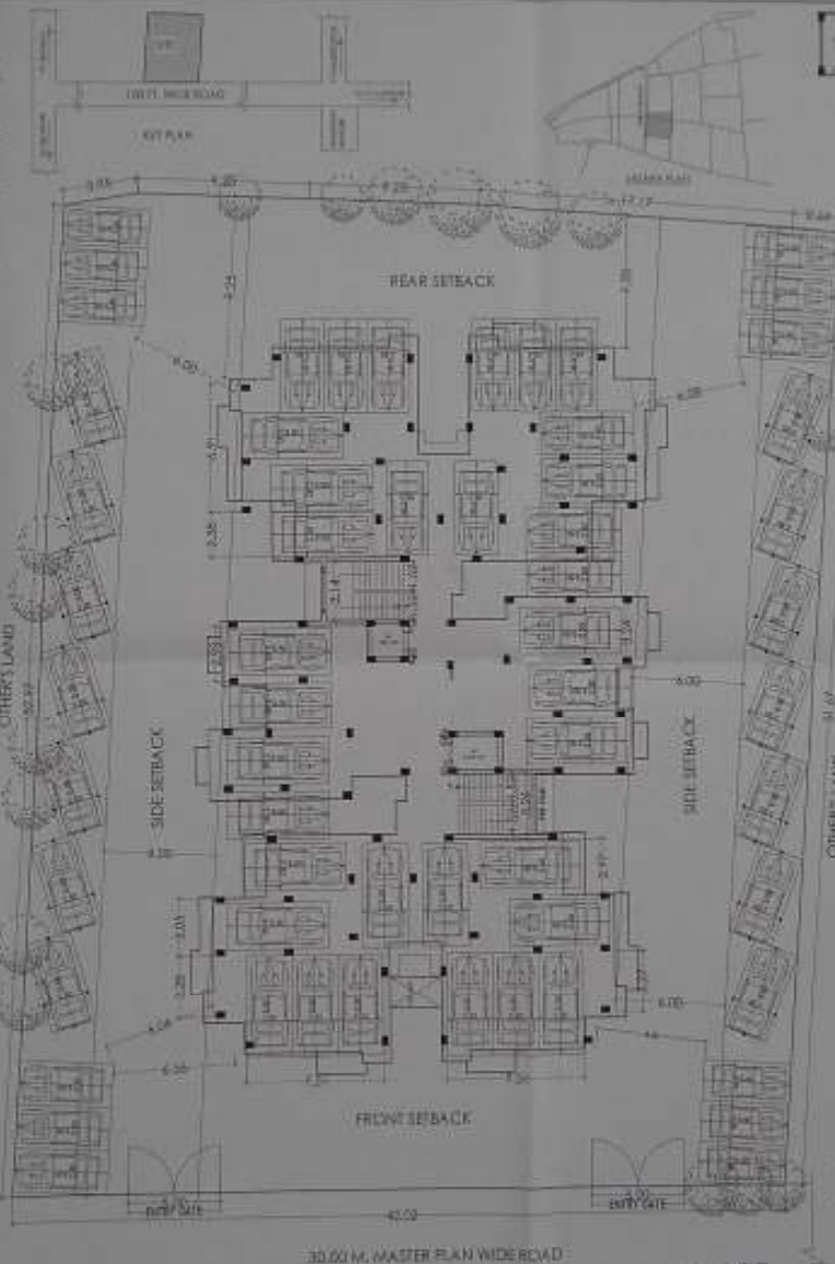
STILT/ GROUND FLOOR PLAN
