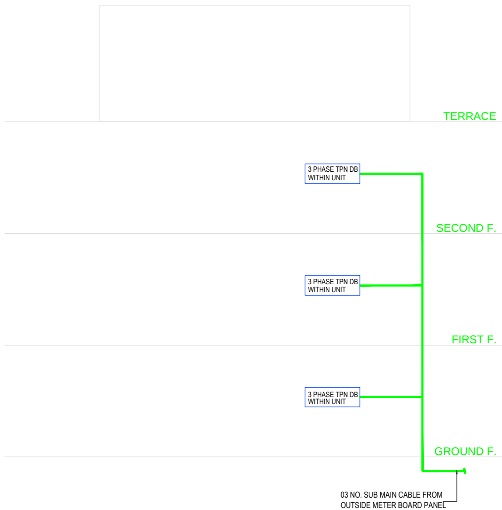
TYPICAL ELECTRICAL SLD FOR FLOORS- WAVE FLOORS
