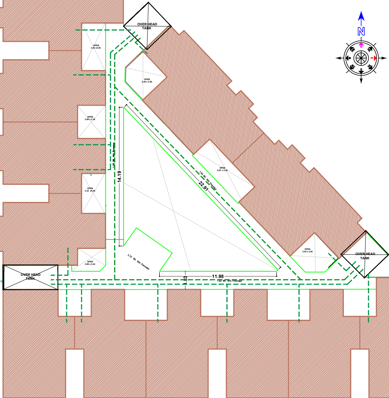
TYPICAL FLOOR PLAN ( 2nd. to 6 th.)
