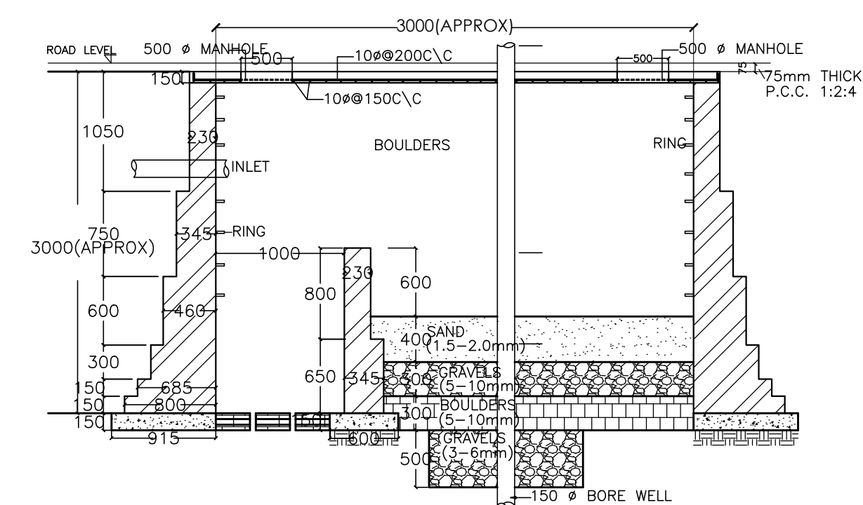
PART SECTION OF RECHARGE STRUCTURE
