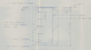
INSPECTION CHAMBER DETAIL FOR SEWER DRAIN
