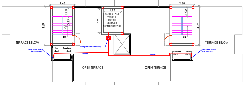
TERRACE FLOOR PLAN-EWS BLOCK (BLOCK B) (SCALE 1:100)
