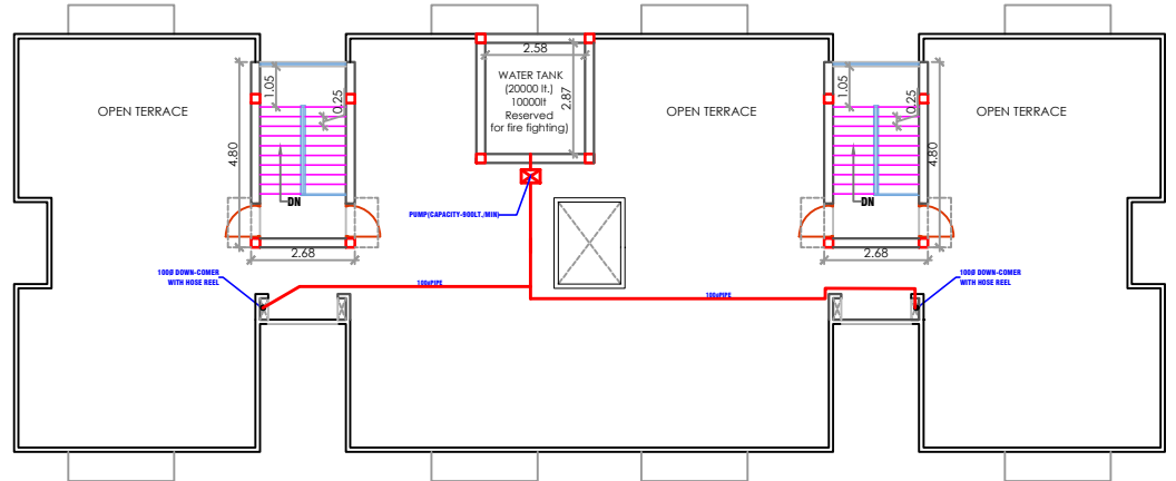
TERRACE FLOOR PLAN-LIG BLOCK (BLOCK A) (SCALE 1:100)
