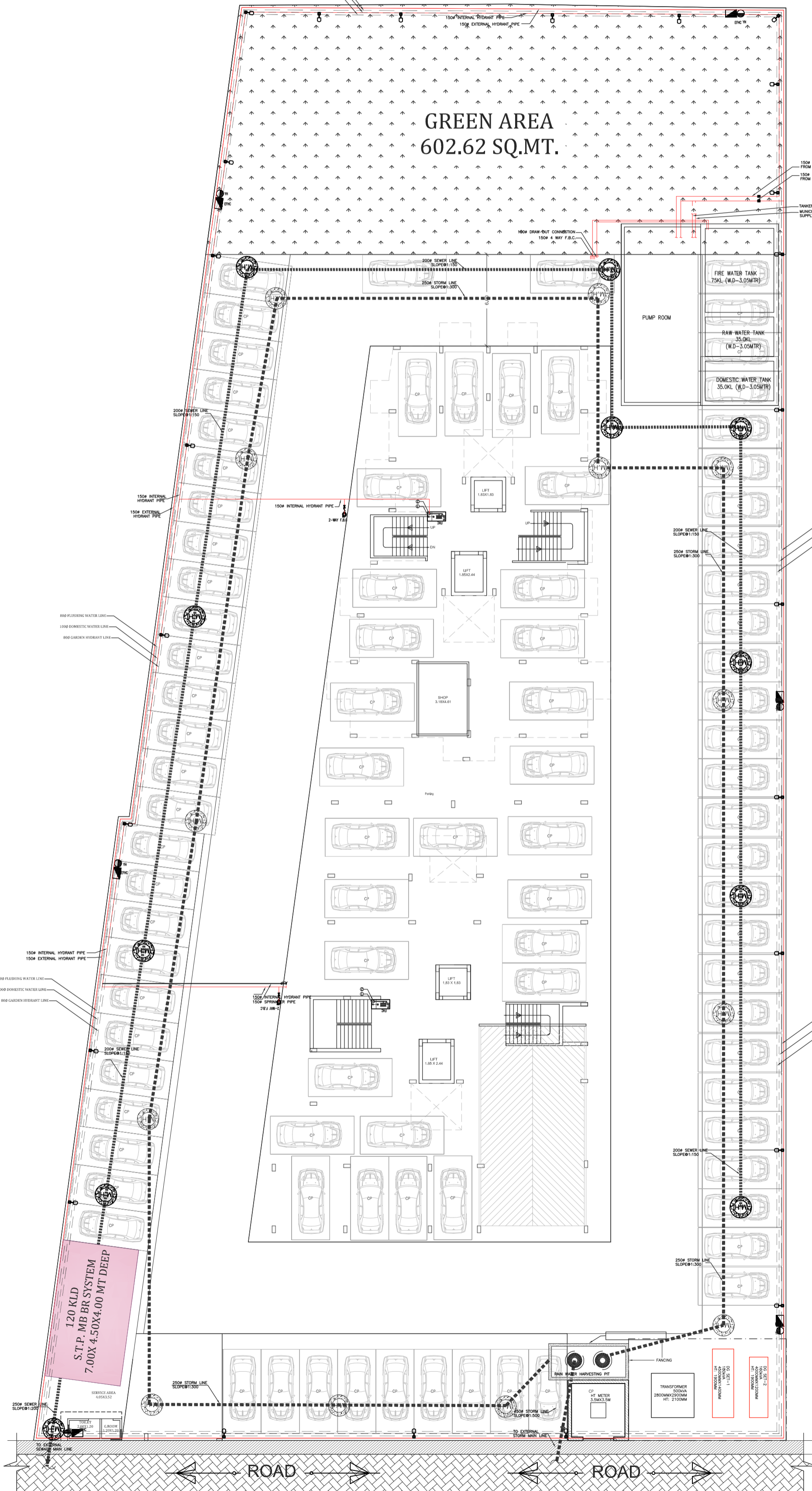
SITE PLAN
