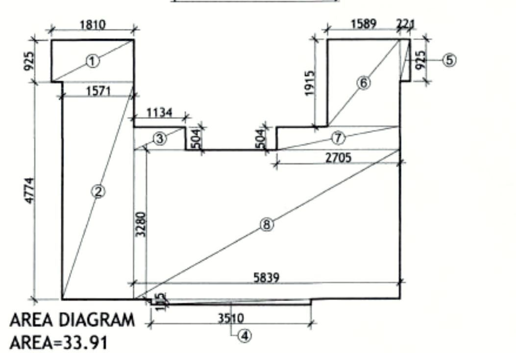
ENT. LOBBY AREA DIAGRAM (GROUND FLOOR)
