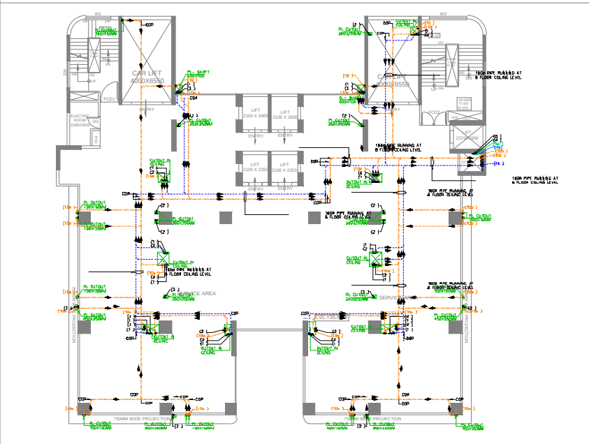
8TH FLOOR PLAN (SERVICE FLOOR)
