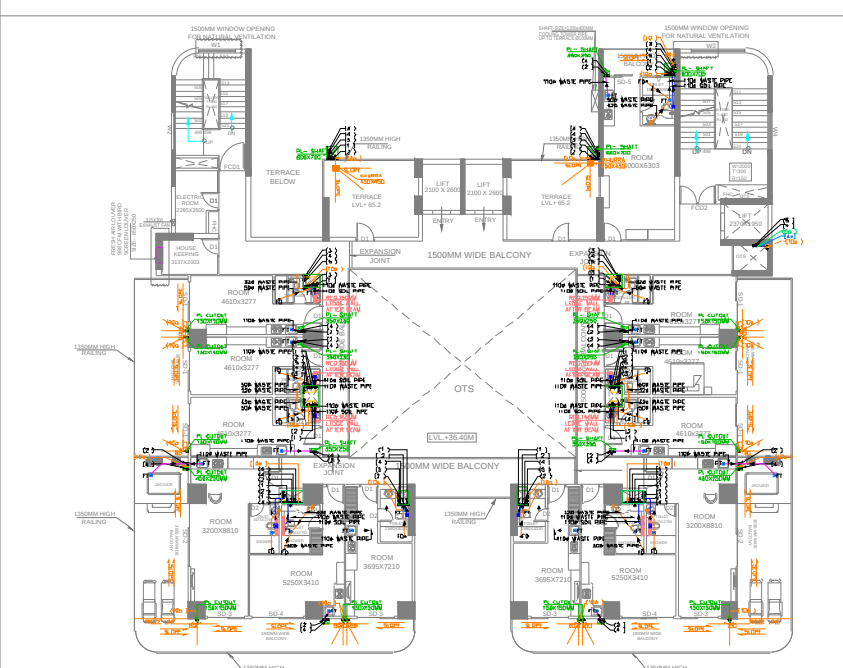
17TH FLOOR PLAN
