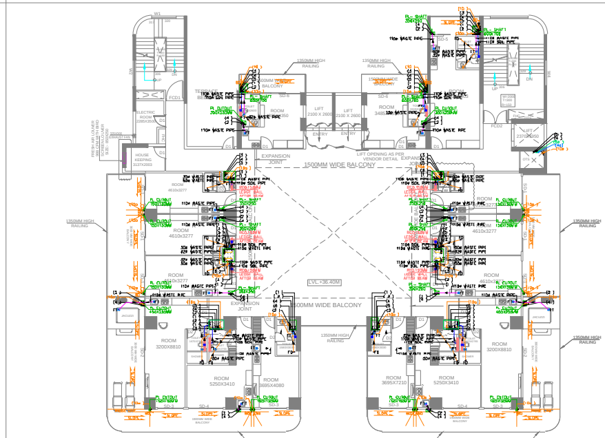
10TH FLOOR PLAN
