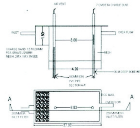
PLAN OF RAIN WATER HARVESTING
