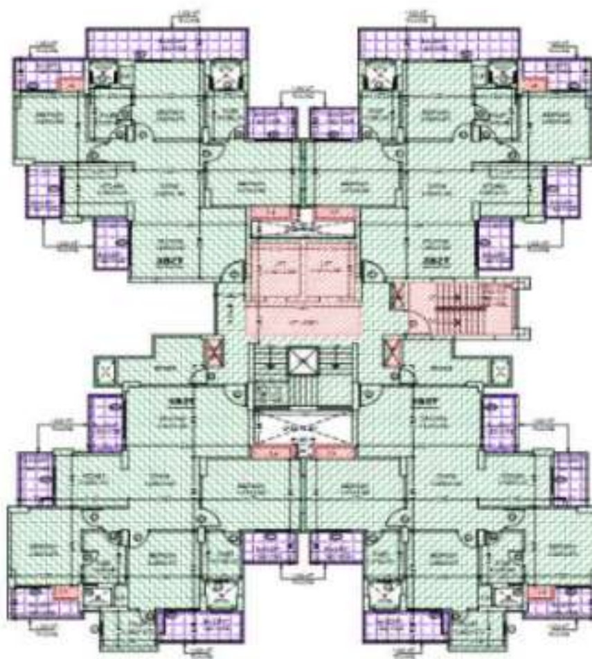
12TH FLOOR PLAN
