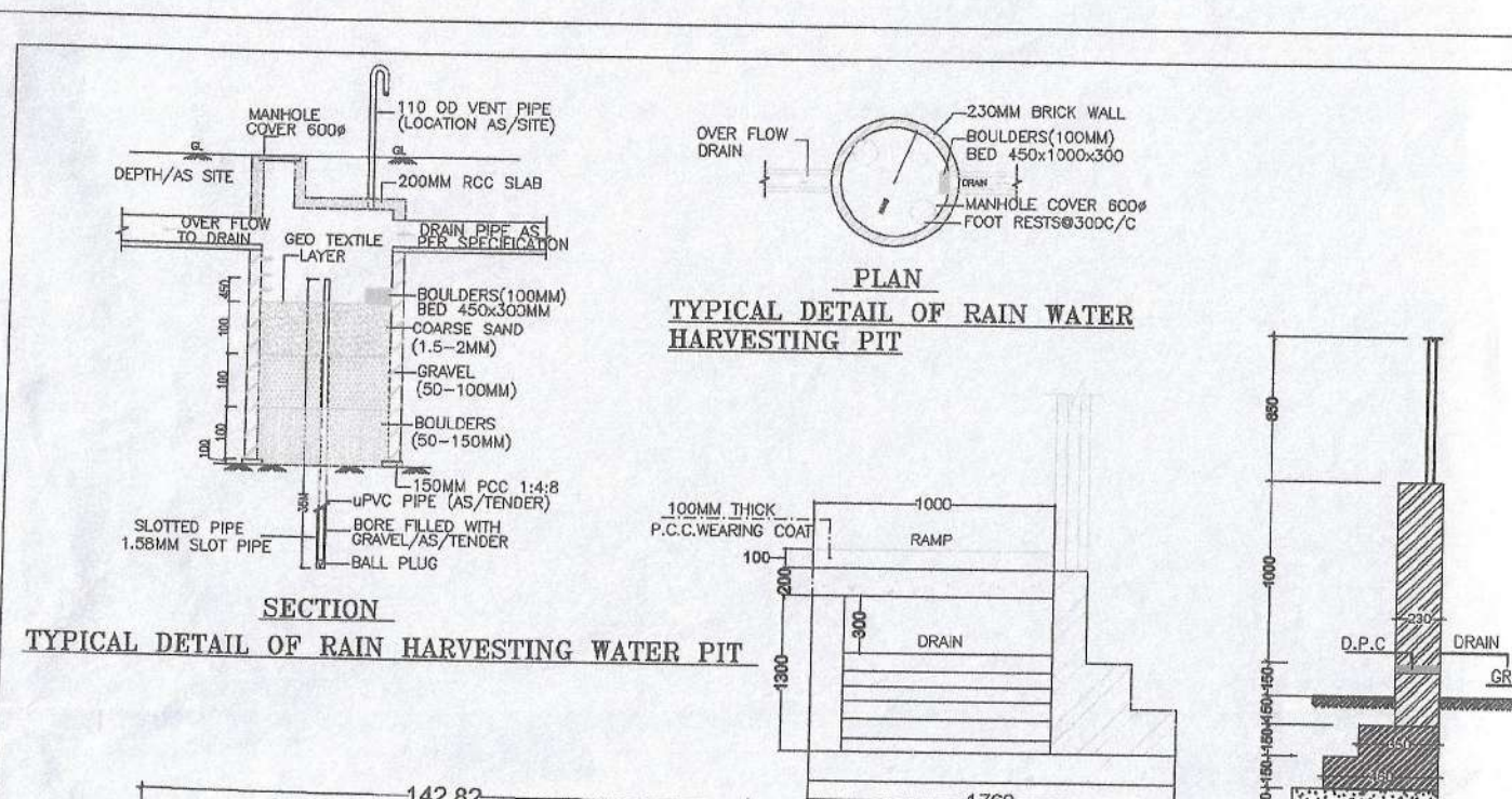
PLAN TYPICAL DETAIL OF RAIN WATER HARVESTING PIT SECTION TYPICAL DETAIL OF RAIN WATER HARVESTING PIT
